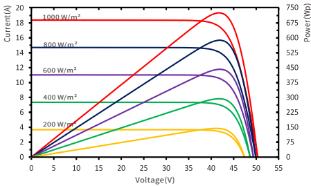
RSM132-8-730BHDG I-V characteristics at different irradiances
