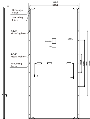
Dimensions of PV Module Unit: mm
